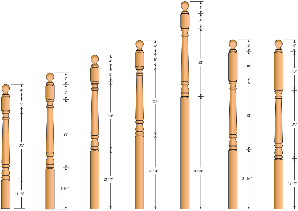
4010BT-44 3" Newel Post 4010BT-48 3" Newel Post 4012BT-54 3" Newel Post 4012BT-59 3" Newel Post 4012BT-72 3" Newel Post 4015BT-59 3" Landing Newel 4015BT13FC-59 3" Landing Newel
