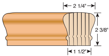
6010 Bending Rail (7 piece)
