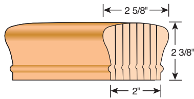
6210 Bending Rail (9 piece)
