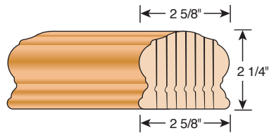
8200 Bending Rail (8 piece)
