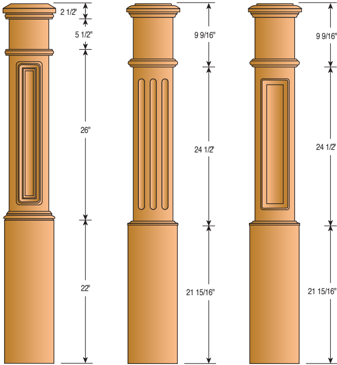
993-56 7 1/2" Box Newel
